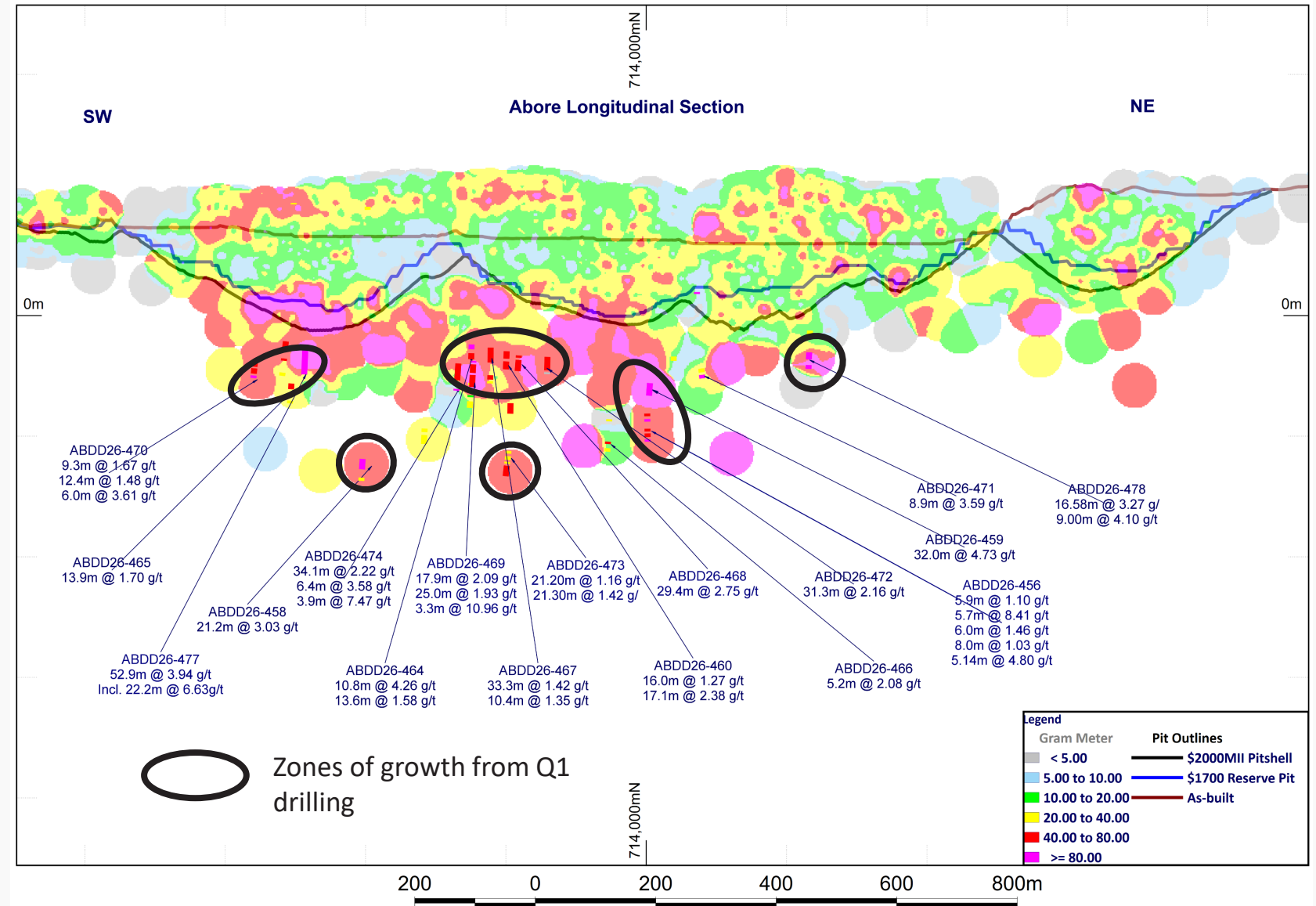
Above long section showing gram meter contours, including results from Q1 drilling
