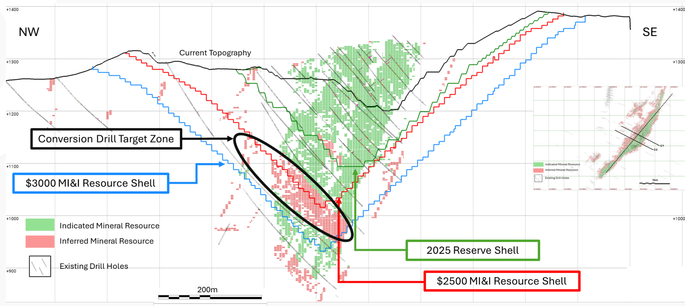
Example cross section through Esaase Main pit showing Inferred and Indicated Resources, growth potential at various gold prices, and conversion target zone
