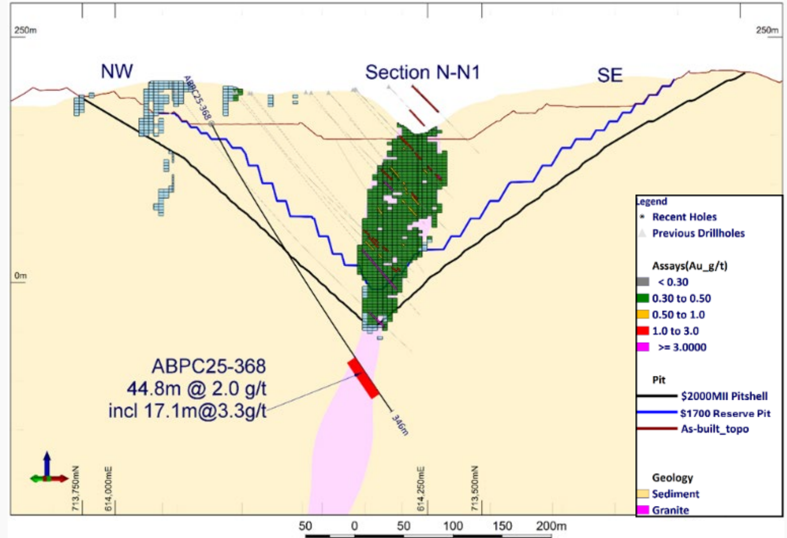
Cross Section N-N1 showing hole ABPC25-368
