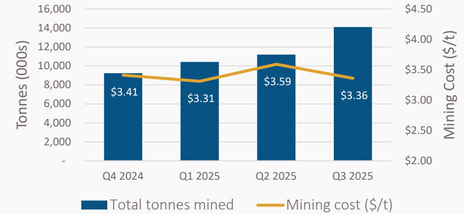
Mining Cost per Tonne and Total Tonnes Mined Trailing 4 Quarters
